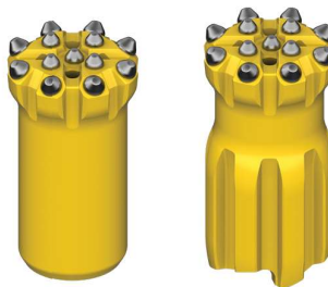
Powerface bit Trubbnos buttons, heavy duty (HD)
