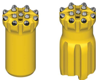
Powerface bit Trubbnos buttons
