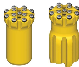
Powerface bit Spherical buttons, standard or heavy duty (HD)
