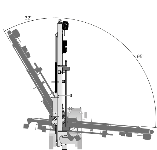
Feed swing angles - standard feed
