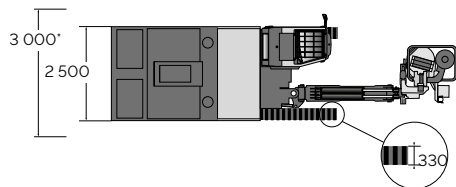
Width (mm) (*with wide kit option)
