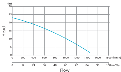
Performance curve
